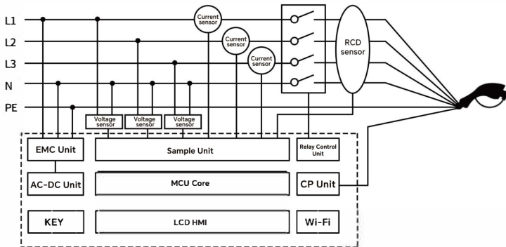
Fig.2 Electrical schematic diagram
